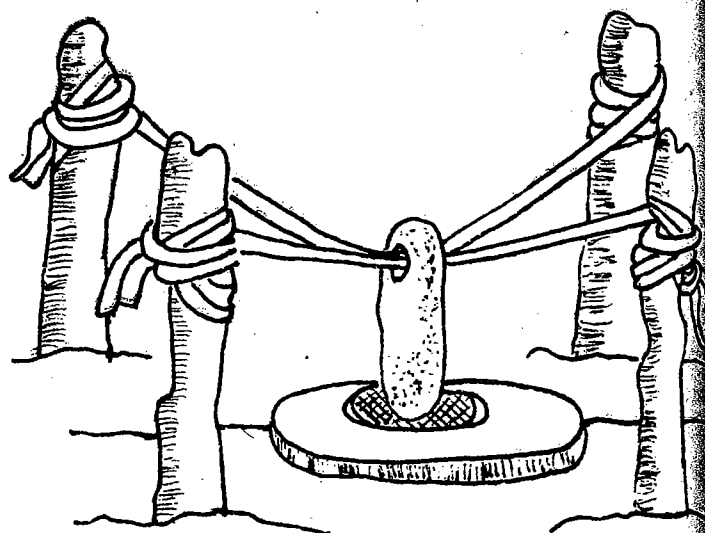
4. PESTLE *SUSPENDED ABOVE MORTAR BY ROPES.
